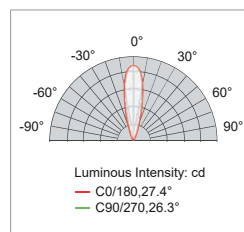
MINITRACK SPOTS(30°)
