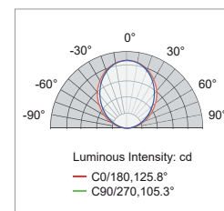
MINITRACK LINEAR(125°)
